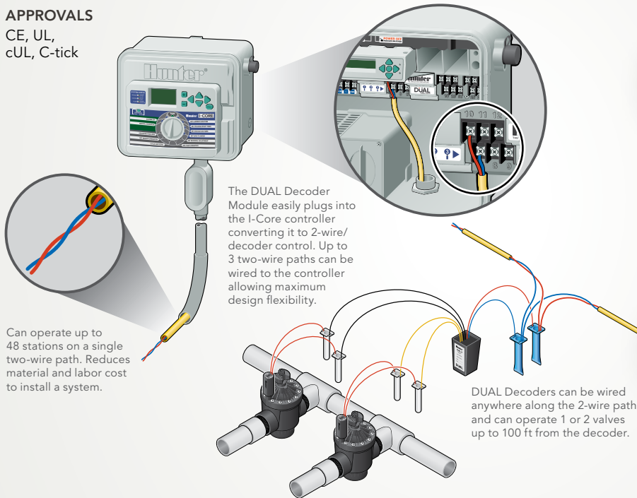
DUAL decoders and surge arrester: 3" H x 1¾" W x 2" D
